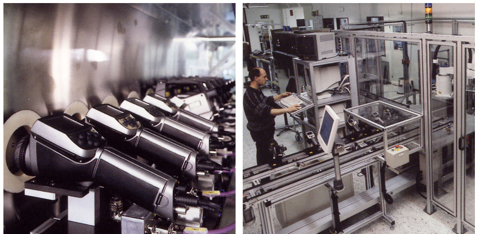
Figure 28.5 LEFT: Testing of infrared cameras in the climatic chamber; RIGHT: Robot used for camera testing and calibration
